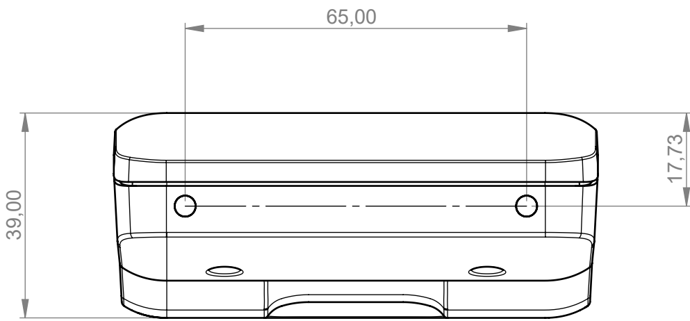
Ansicht "Z" View "Z"
