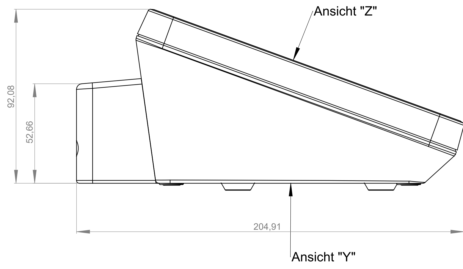
Ansicht "Y" View "Y"
