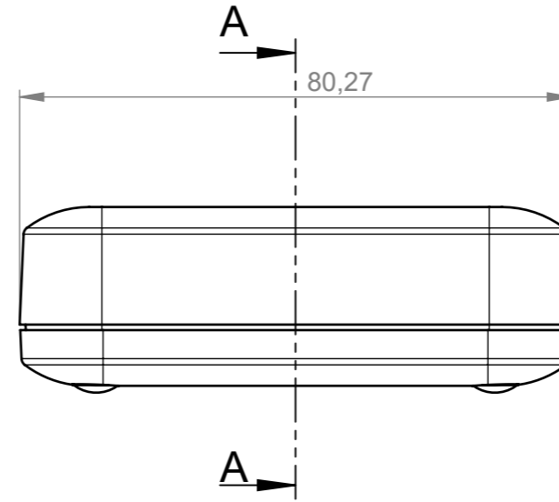
Ansicht "Z" View "Z"
